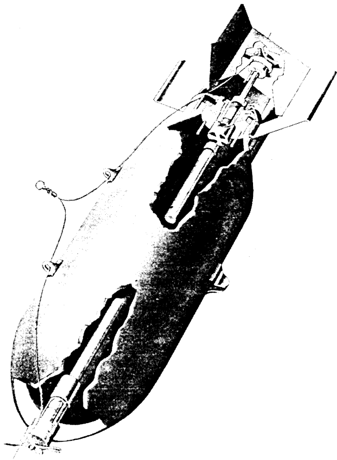
Figure 4.12 500 lb GP Bomb AN M64A1 with Fuze Assembly AN M109A1, Cutaway View.
